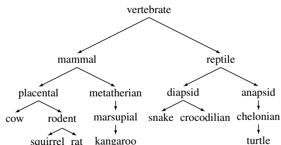
Figure 1: An excerpt of WordNet's vertebrates taxonomy.
